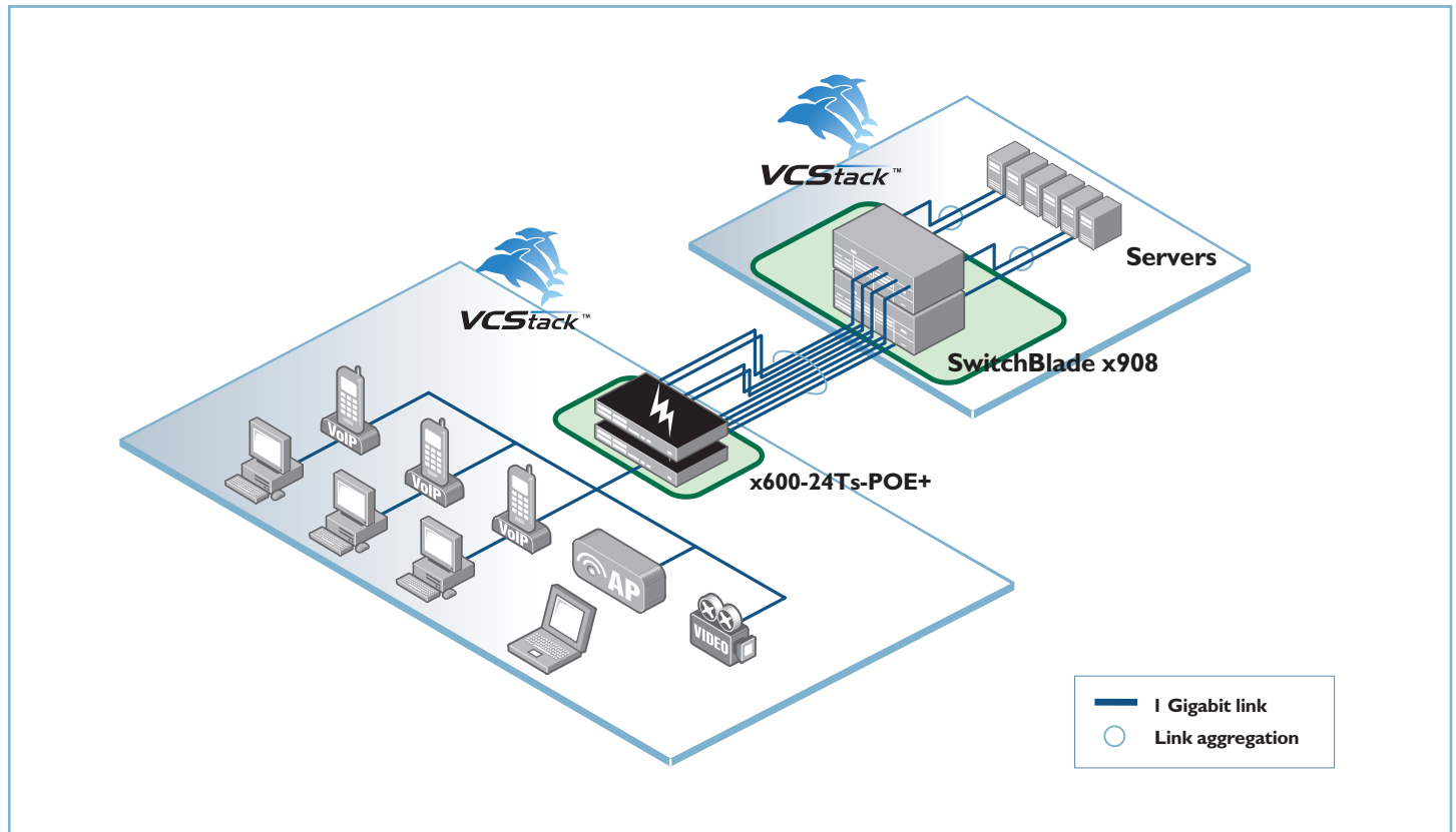
Diagram 1: PoE+ Provision
