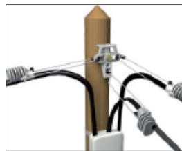
Triple dead-ending (distribution poles)
