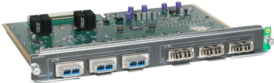
Figure 5. Cisco TwinGig Converter Module converts each 10 Gigabit Ethernet X2 Interface into Two Gigabit Ethernet SFP Ports with Catalyst 4500 E-Series 6-port 10 Gigabit Ethernet Linecard
